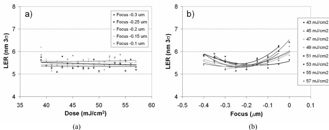
Figure 6. TOK N023 LER behavior through (a) dose and (b) focus
