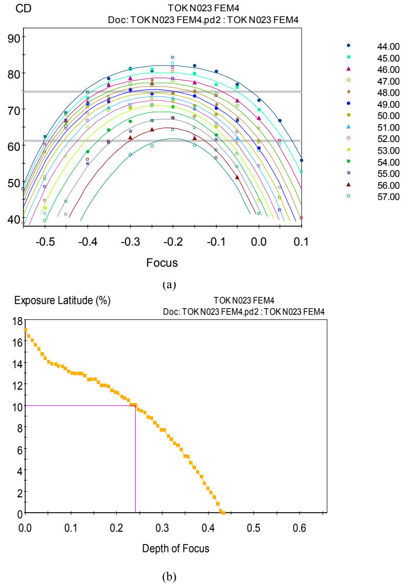
Fig. 4 Process window analysis for TOK N023; (a) Bossung curve and (b) exposure latitude vs. DoF
